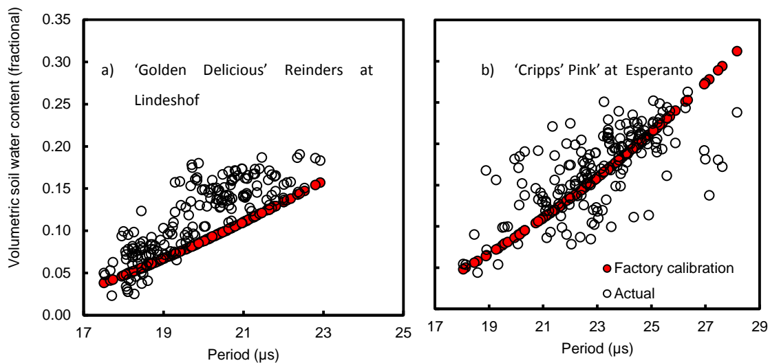
Fig. 4.6 Comparison of CS616 factory calibrated volumetric soil water content and actual volumetric soil water content sampled simultaneously at various CS616 periods at a) Lindeshof) and; b) Esperanto orchards, respectively.
