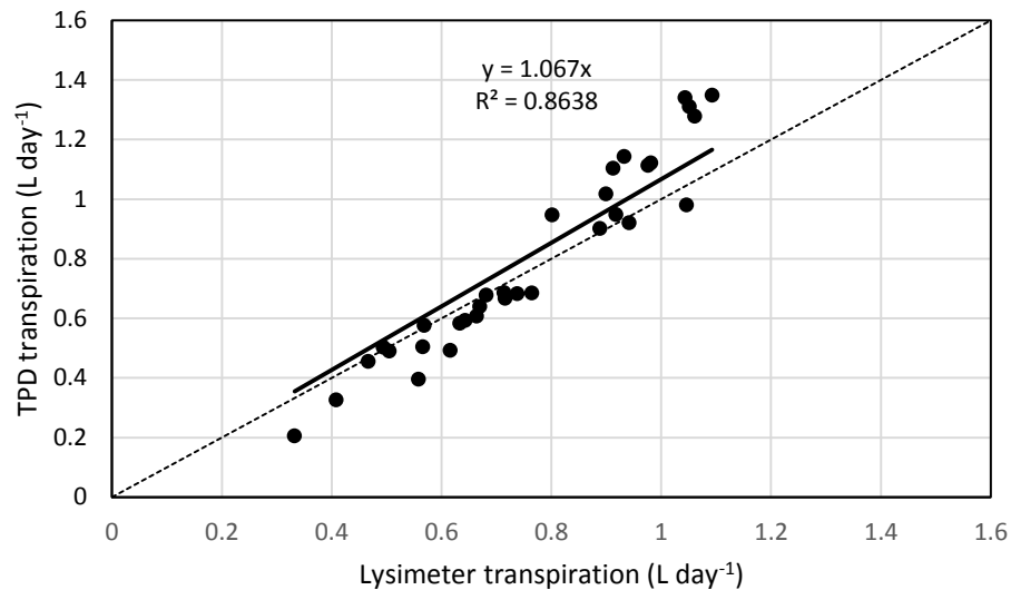
Fig. E5 Calibration of transpiration determined by the thermal dissipation method with transpiration determined using a weighing lysimeter. The 1:1 line is indicated by the dotted line.
