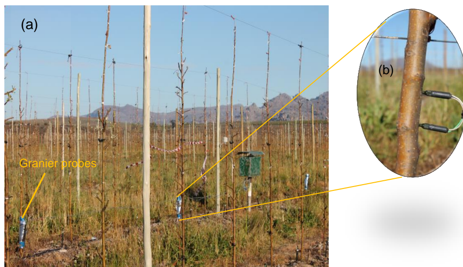
Fig. 3.8 (a) Measurement of transpiration in young orchards using Granier probes. (b) Granier probe installation using 10 mm sensors.
