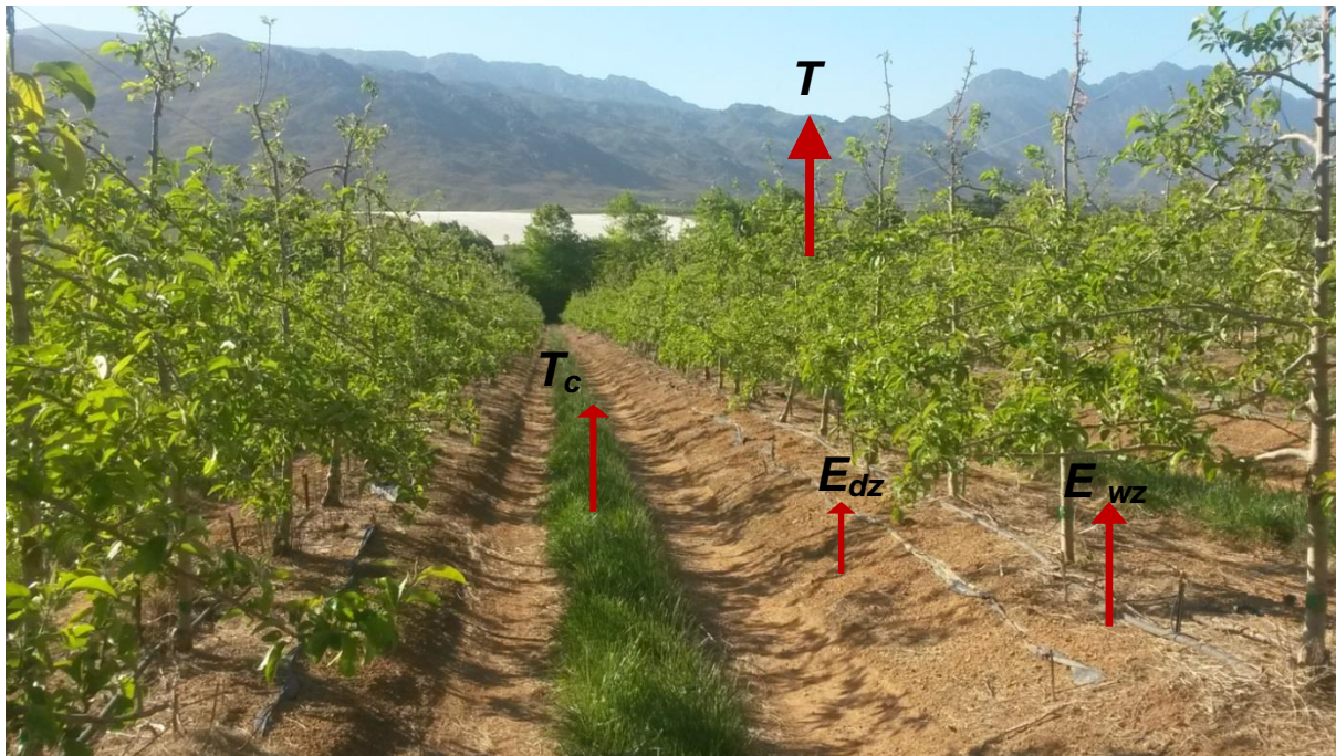
Fig. 2.5 Evapotranspiration components from an orchard under micro-irrigation. T represents the tree transpiration, T_c is the cover crop transpiration, E_{dz} and E_{wz} is the evaporation from the dry and wet soil zones.
