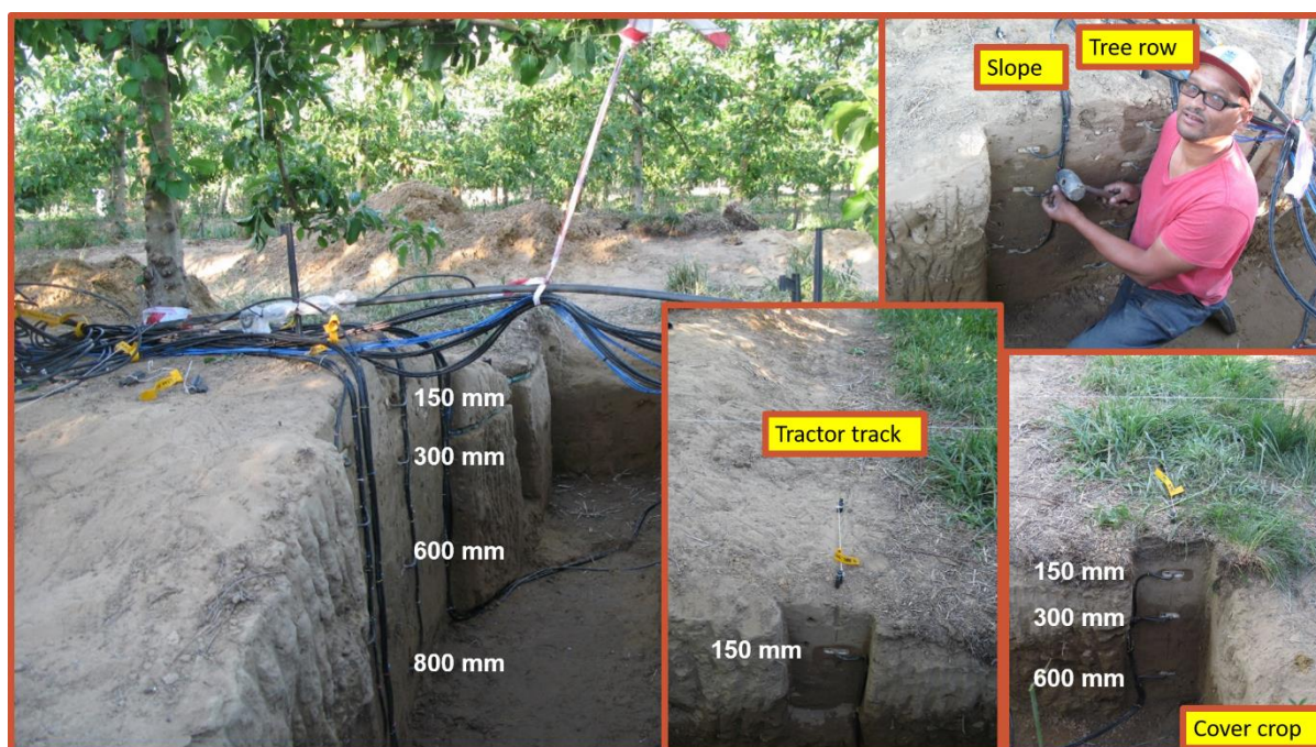
Fig. 4.2 Installation of CS616 sensors in sandy loam soil at various depths in the tree row, ridge, slope, tractor track and cover crop area in the medium canopy cover 'Cripps' Pink' orchard at Esperanto in 2016/17.
