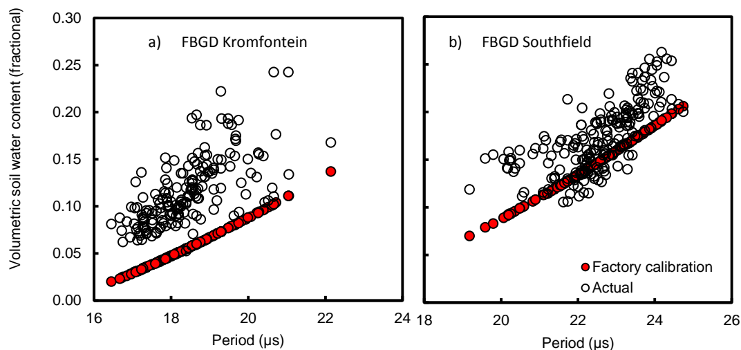
Fig. 5.5 Comparison of CS616 factory calibrated volumetric soil water content and actual volumetric soil water content sampled simultaneously at various CS616 periods at the FBGD orchards at a) Kromfontein and b) Southfield.
