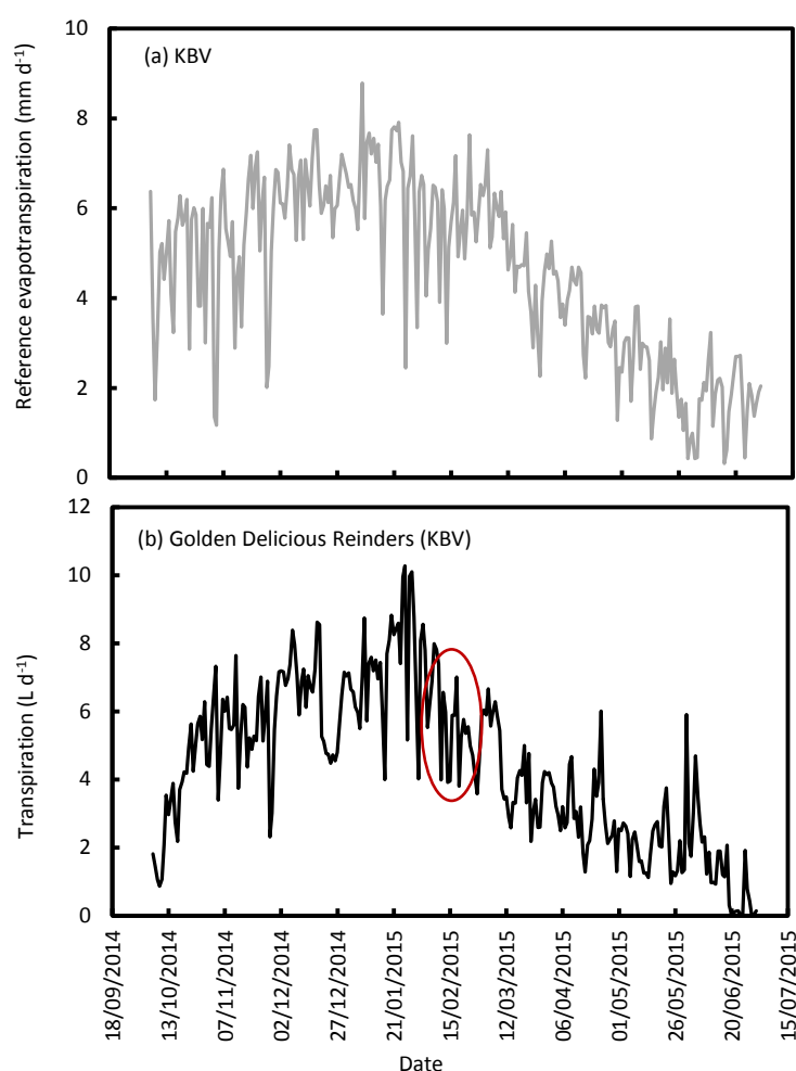
Fig. 3.18(a) Seasonal evapotranspiration trend in KBV during the 2014/15 season. (b) Daily transpiration dynamics of a young non-bearing ‘Golden Delicious Reinders’ from 01 October 2014 to 30 June 2015. Red circle indicate a period of water stress.
