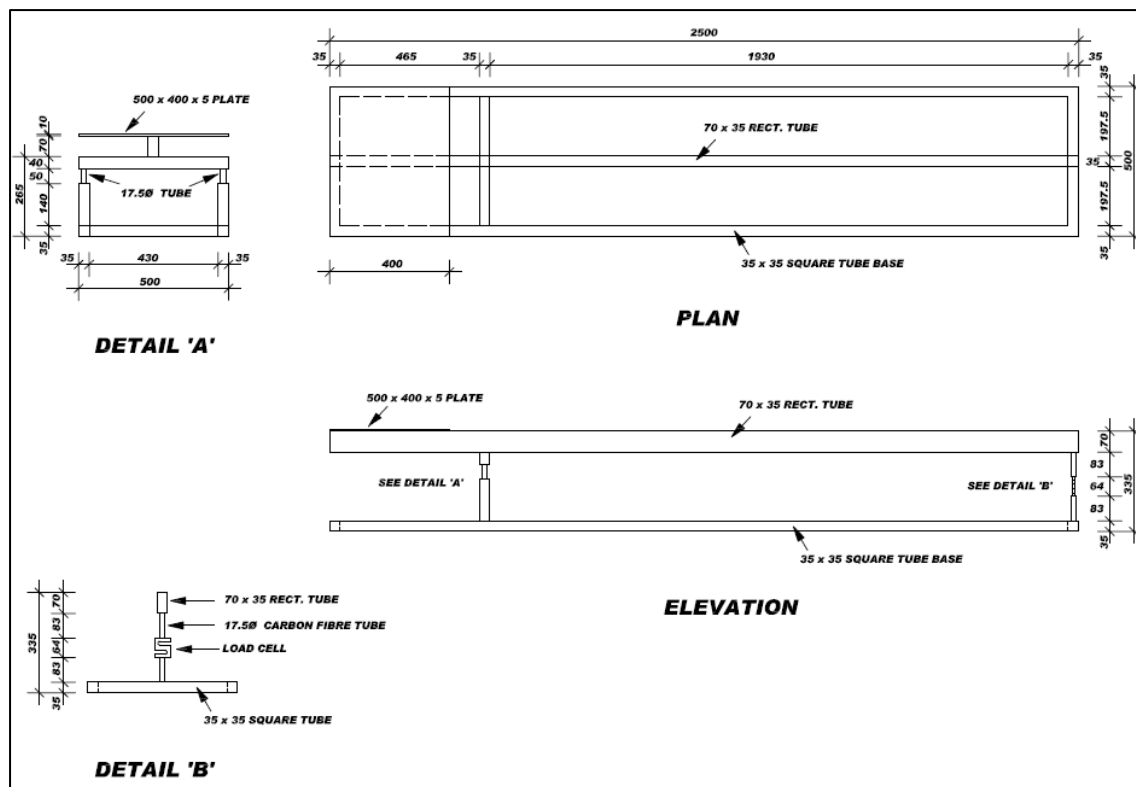
Fig. E1 Detailed sketch of the cantilever weighing lysimeters
