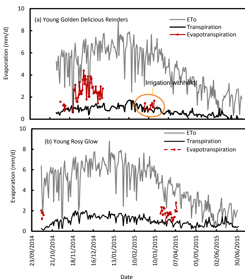
Fig. 3.24 Comparison of measured transpiration (bold black lines), actual evapotranspiration (red lines) and the short grass reference evapotranspiration (grey line) for: (a) young non-bearing ‘Golden Delicious Reinders’; (b) young non-bearing ‘Rosy Glow’ orchards in KBV during the 2014/15 season.
