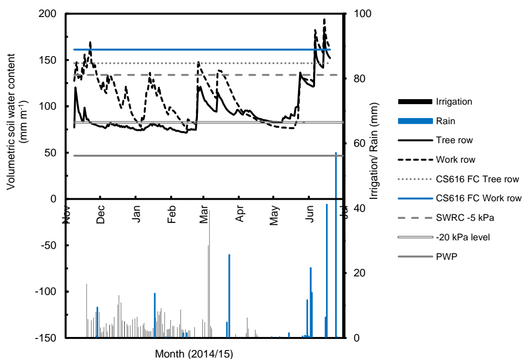
Fig. 5.6 Seasonal changes in volumetric soil water content in the tree row and work row areas of a full-bearing 'Golden Delicious' orchard at Kromfontein in the Koue Bokkeveld during the 2014/15 season. The amount of irrigation applied over the full surface area and rainfall received are indicated on the Y-axis.
