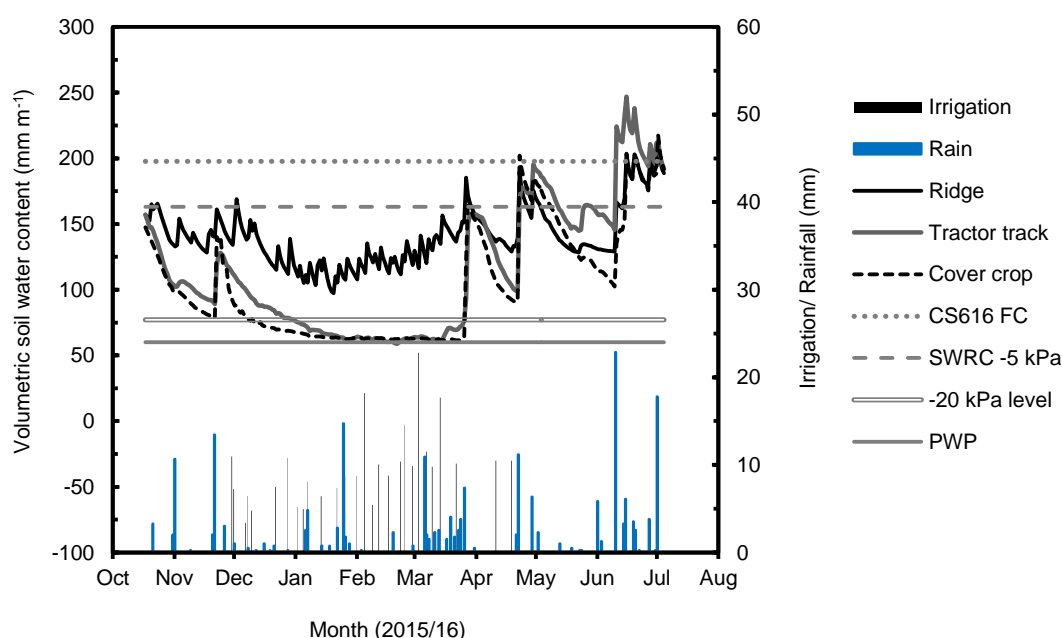
Fig. 3.15 Seasonal changes in volumetric soil water content in the ridge, tractor track and cover crop areas of a non-bearing 'Cripps' Red' orchard at Vyeboom in EGVV during the 2015/16 season. The amount of irrigation applied to the ridge and rainfall received are indicated on the Y-axis.
